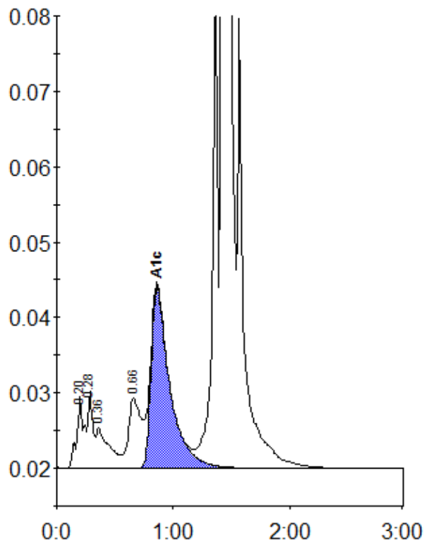
Peak table - ID: 10547191
